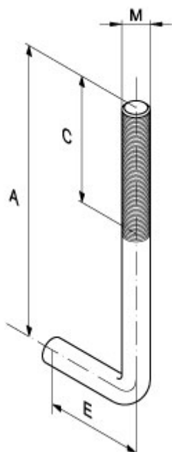
Fig.120 Haakanker, RVS-304
