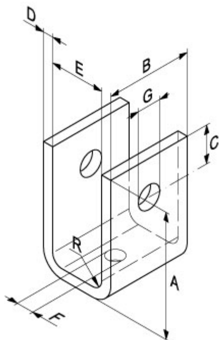
Fig.140 Ophangbeugel, S235 zwart
